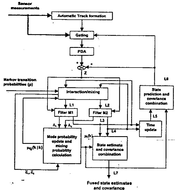
Fig.1 A 2-model IMM PDAF scheme
